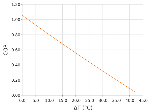
Coefficient of Performance (COP = Q_c/P_{in} ) Voperating = 12 Volts | Ioperating = 5.1 Amps
