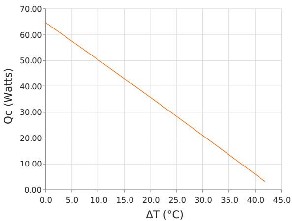
Heat Pumped at Cold Side ( Q_c ) Voperating = 12 Volts | Ioperating = 5.1 Amps
