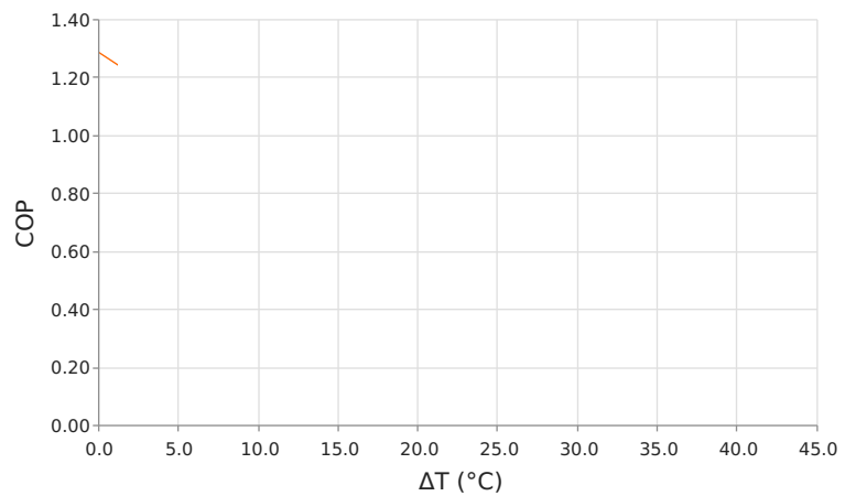
Coefficient of Performance (COP = Q_c/P_{in} ) V_{operating} = 24 Volts | I_{operating} = 4.36 Amps
