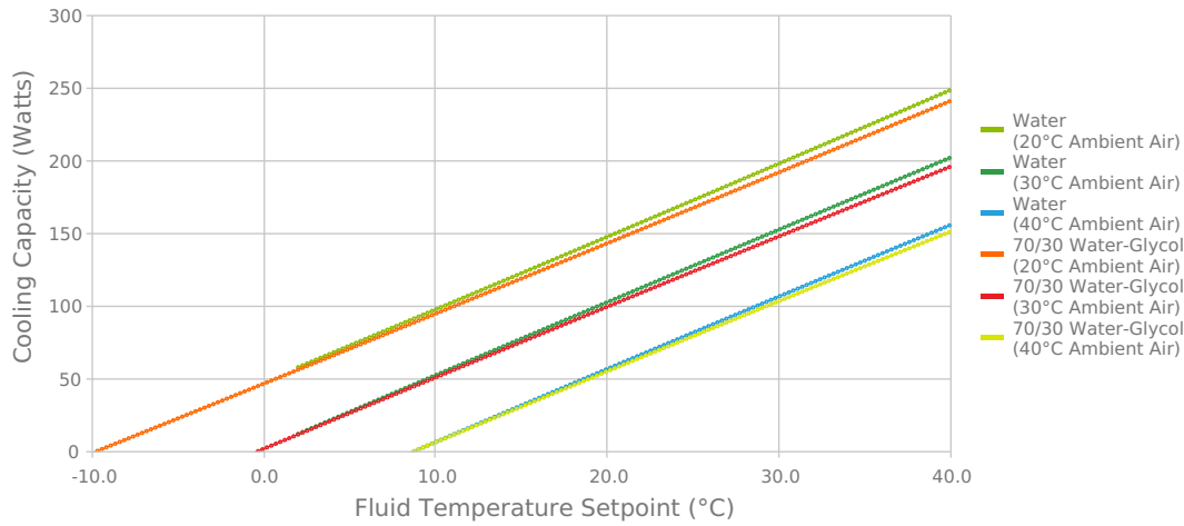
MRC150-DH2-HT-DV Cooling Capacity (Qc)
