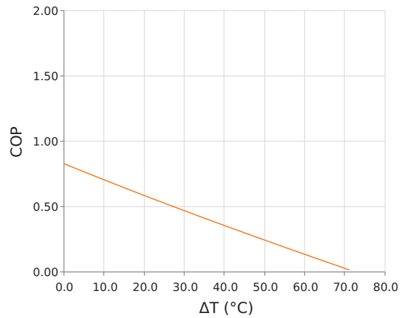
Coefficient of Performance (COP = Qc/Pin) Thot = 35 °C | Ioperating = 3.4 Amps
