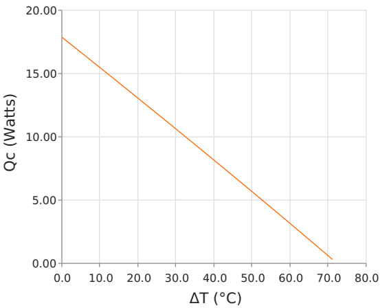
Heat Pumped at Cold Side (Qc) Thot = 35 °C | Ioperating = 3.4 Amps
