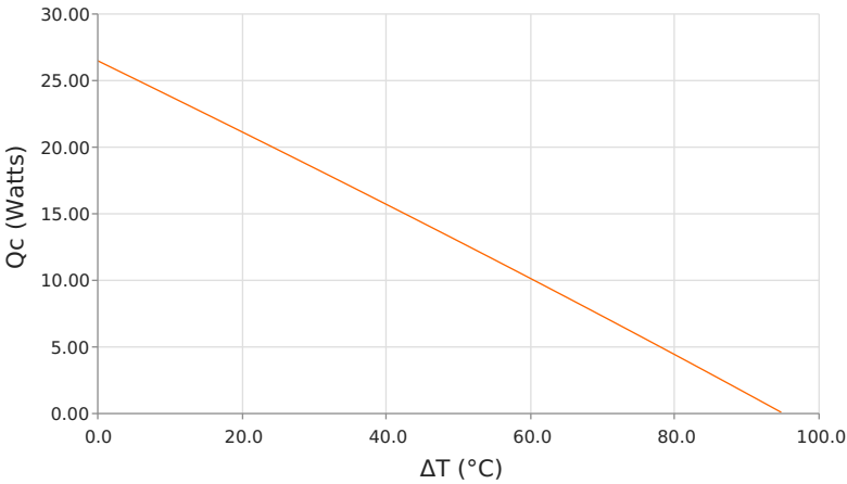
Heat Pumped at Cold Side ( Q_c ) T_{hot} = 35^\circ\text{C} | i_{operating} = 8.2 Amps
