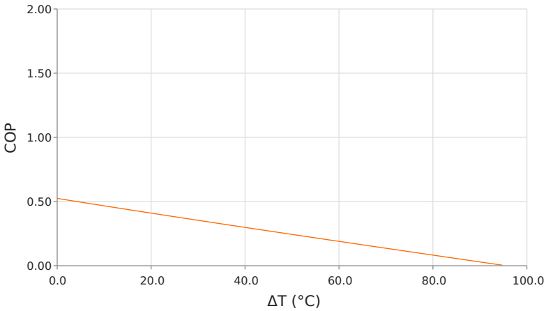
Coefficient of Performance (COP = Q_c/P_{in} ) T_{hot} = 35^\circ\text{C} | i_{operating} = 8.2 Amps
