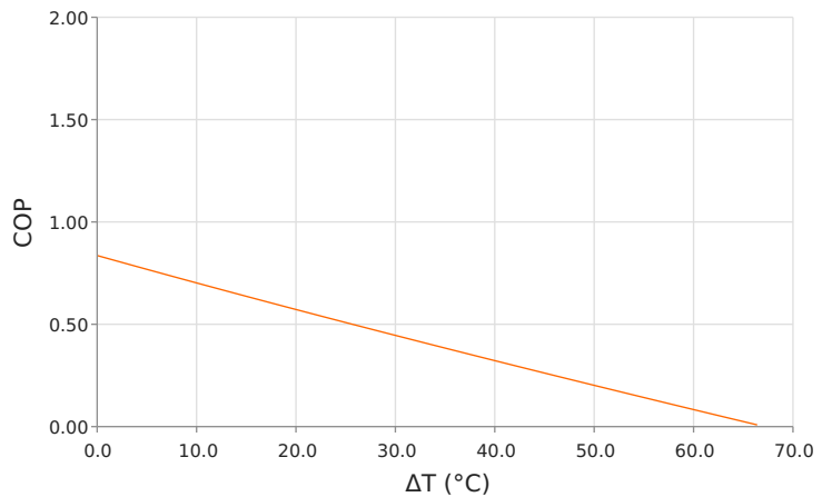
Coefficient of Performance (COP = Q_c/P_{in} ) T_{hot} = 27^\circ\text{C} | Current = 0.7 Amps
