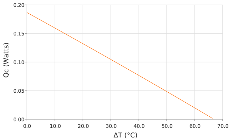
Heat Pumped at Cold Side ( Q_c ) T_{hot} = 27^\circ\text{C} | Current = 0.7 Amps
