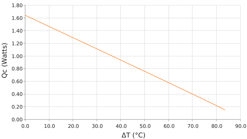
Heat Pumped at Cold Side ( Q_c ) T_{hot} = 85^\circ\text{C} | operating = 1 Amps
