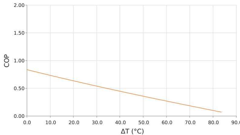
Coefficient of Performance (COP = Q_c/P_{in} ) T_{hot} = 85^\circ\text{C} | operating = 1 Amps
