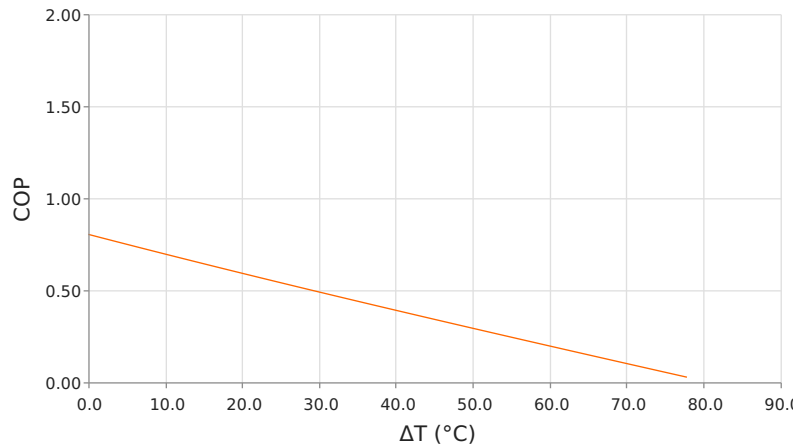
Coefficient of Performance (COP = Q_c/P_{in} ) T_{hot} = 50^\circ\text{C} | operating = 1.3 Amps
