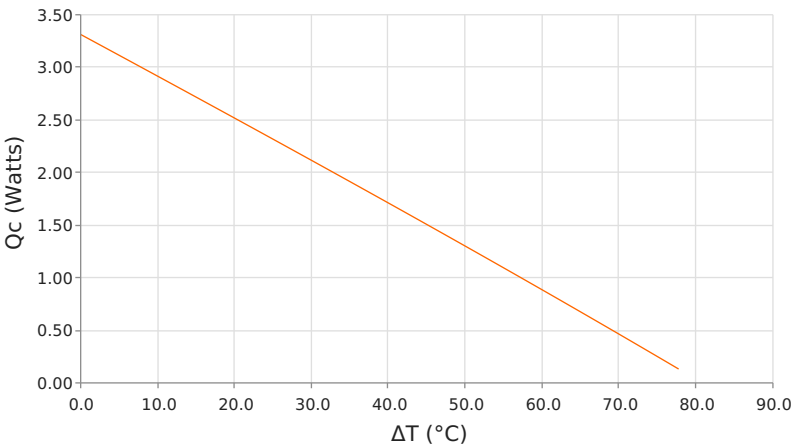
Heat Pumped at Cold Side ( Q_c ) T_{hot} = 50^\circ\text{C} | operating = 1.3 Amps
